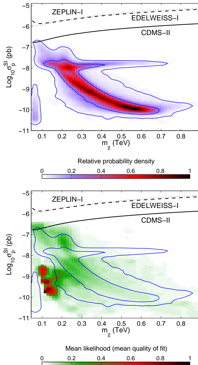
Figure 13: Top panel: the 2-dimensional relative probability density p(m_\chi, \sigma_p^{SI}|d) , with the contours containing 68% and 95% probability also marked. Bottom panel: the mean quality of fit (likelihood) with the same 68% and 95% probability contours as in the top panel to facilitate the comparison. Current 90% experimental upper limits are also shown.
