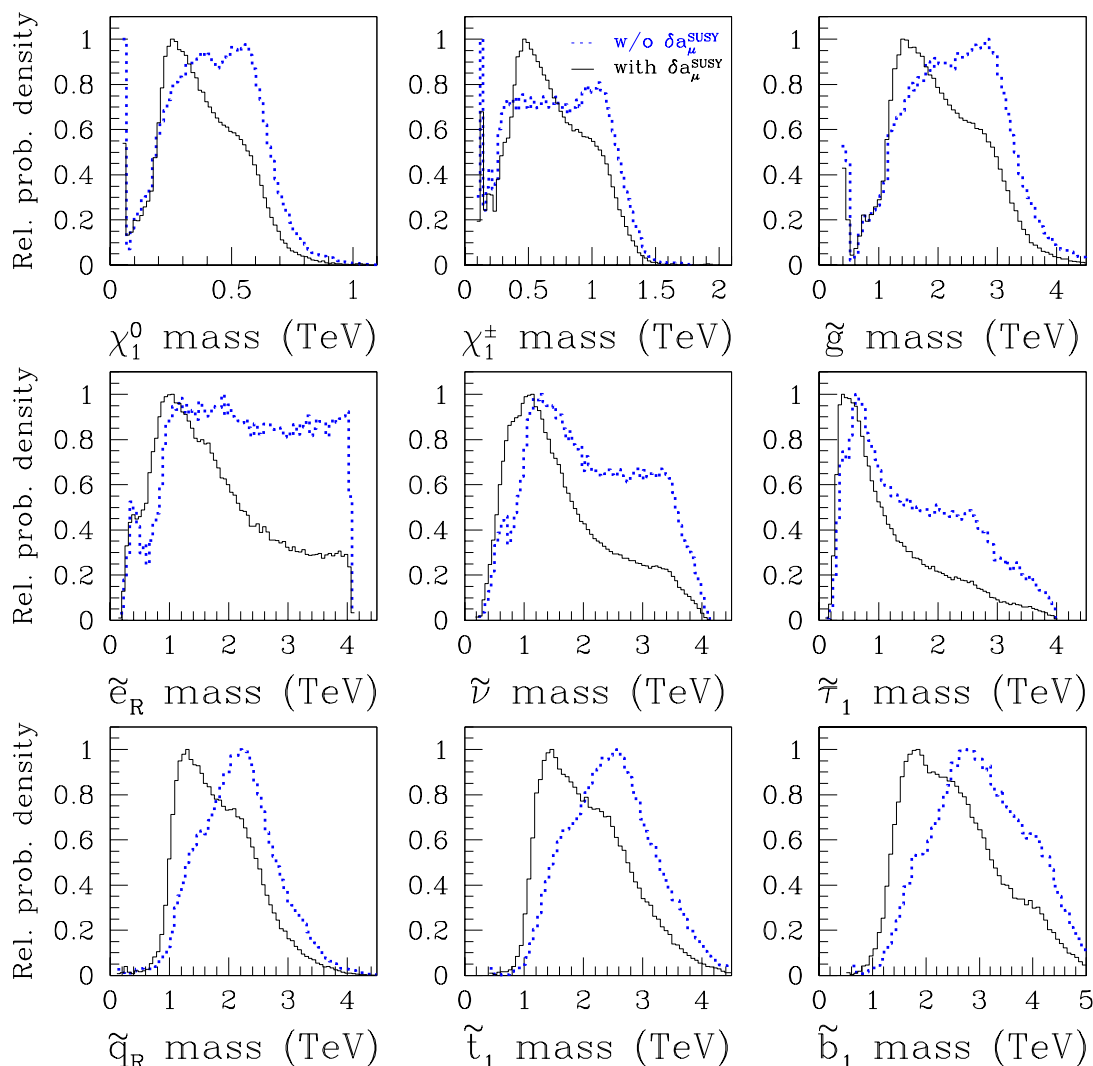
Figure 17: As in figure 5. The black solid (blue dotted) line is for the analysis including (excluding) the measurement of the anomalous magnetic moment of the muon, eq. (3.7). Both cases assume the “4 TeV range” priors.
