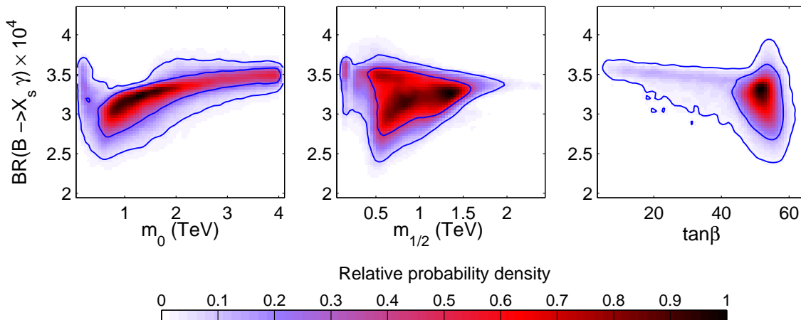
Figure 8: As in figure 6, but for BR(\bar{B} \rightarrow X_s \gamma) . The measured value of BR(\bar{B} \rightarrow X_s \gamma) , eq. (3.8), has been included.
