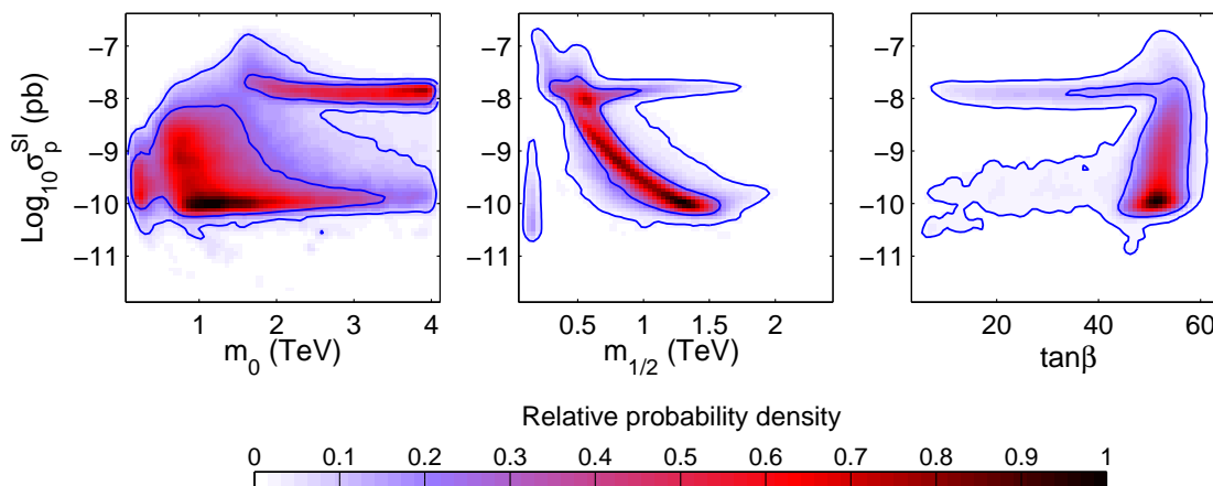
Figure 12: As in figure 6, but for \sigma_p^{SI} .
