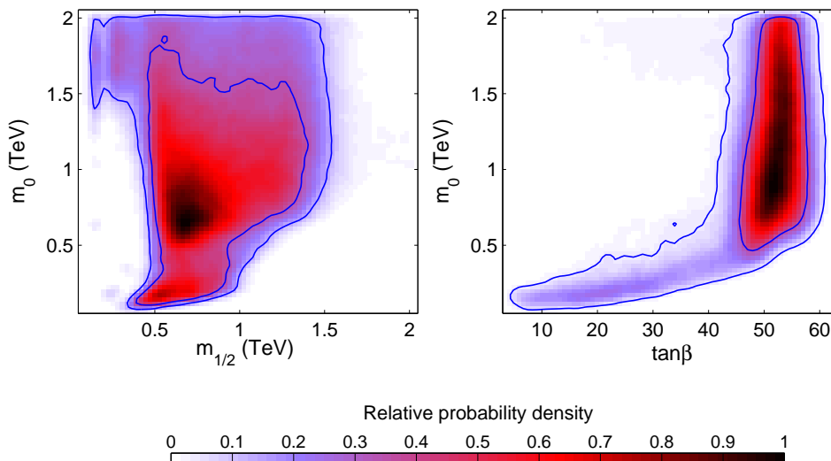
Figure 3: The 2-dimensional relative probability densities as in figure 2 but for the “2 TeV range” analysis and for the planes (m_{1/2}, m_0) and (\tan \beta, m_0) only. Imposing a prior range m_0 < 2 TeV modifies substantially the inferences about the high probability regions for m_0 .
