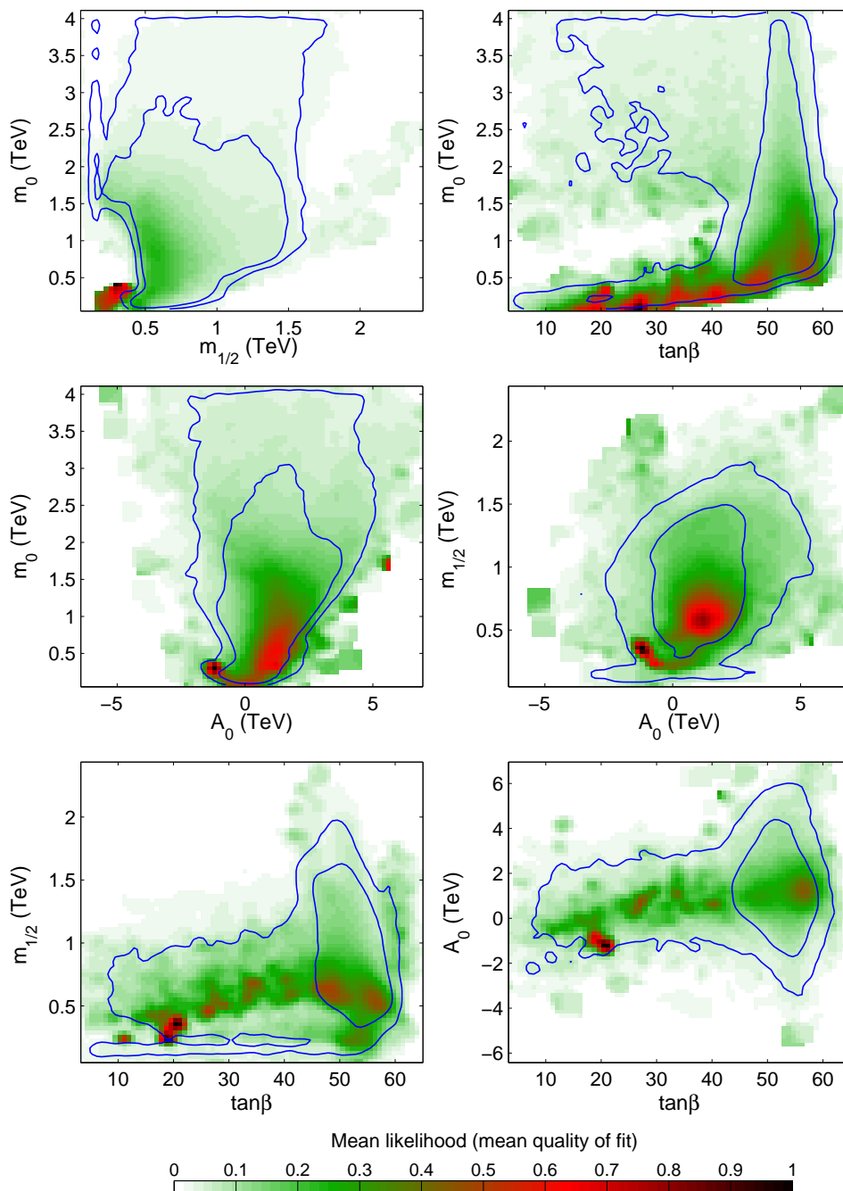
Figure 11: The quality of fit in the planes spanned by the CMSSM parameters: m_{1/2} , m_0 , A_0 and \tan\beta for the “4 TeV range” scan. This figure should be compared with figure 2 where the relative 2-dim joint relative probabilities are plotted for the same pairs of variables.
