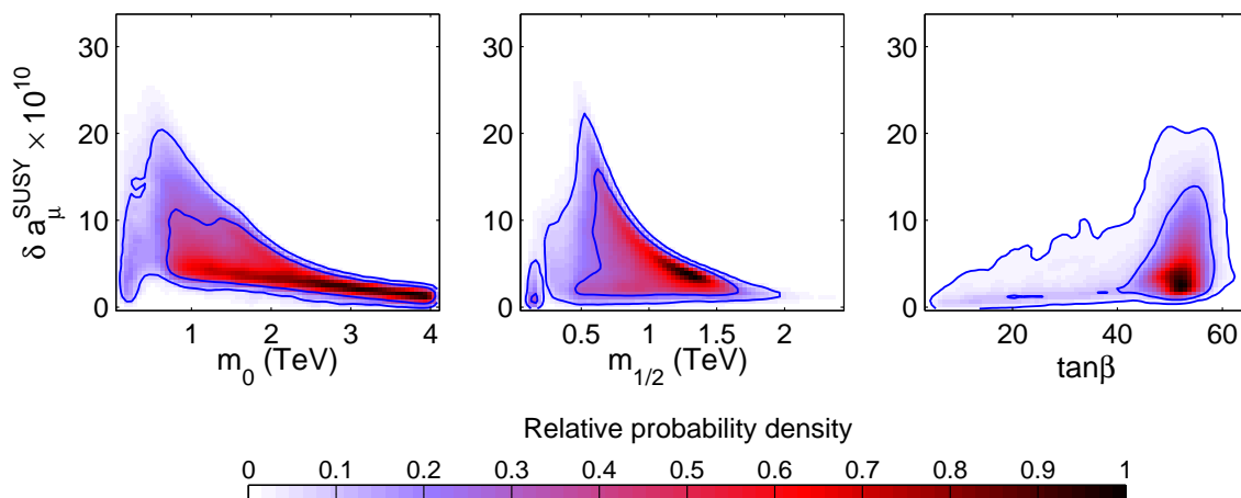
Figure 7: As in figure 6, but for \delta a_\mu^{\text{SUSY}} . The measured value of \delta a_\mu^{\text{SUSY}} , eq. (3.7), has been included.
