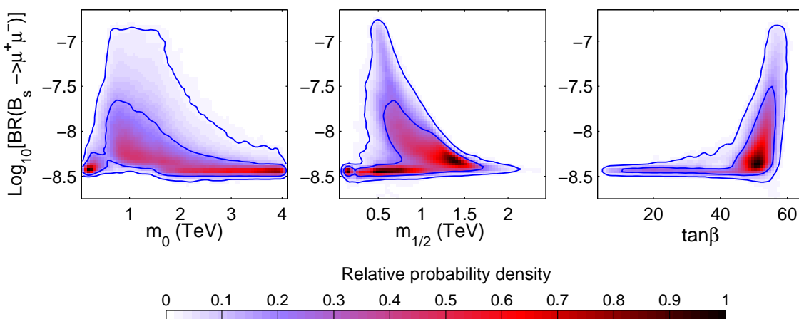
Figure 9: As in figure 6, but for BR(B_s \rightarrow \mu^+ \mu^-) . The upper limit of BR(B_s \rightarrow \mu^+ \mu^-) < 1.5 \times 10^{-7} has been included.
