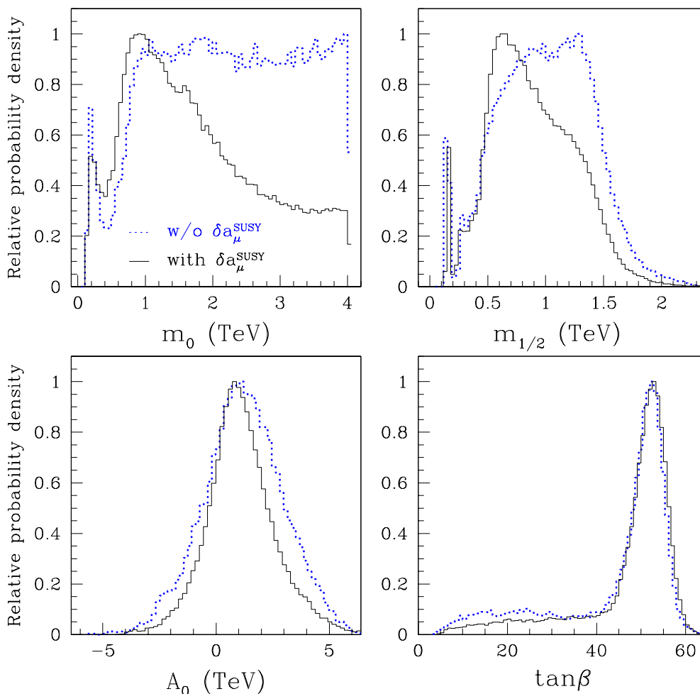
Figure 16: The 1-dimensional relative posterior pdf’s as in figure 4. The black solid (blue dotted) line is for the analysis including (excluding) the measurement of the anomalous magnetic moment of the muon, eq. (3.7). Both cases assume the “4 TeV range” priors.
