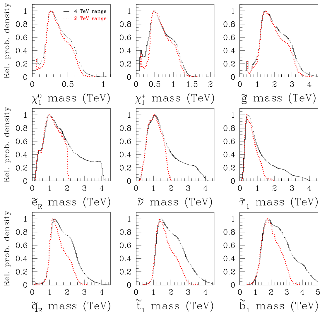
Figure 5: As in figure 4, but for the masses of several representative superpartners.
