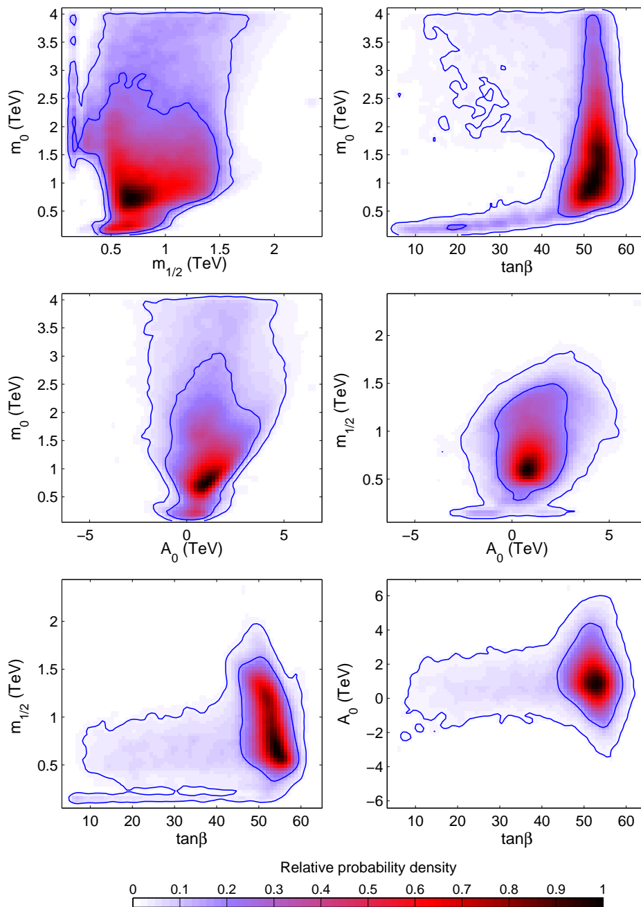
Figure 2: The 2-dimensional relative probability densities in the planes spanned by the CMSSM parameters: m_{1/2} , m_0 , A_0 and \tan\beta for the “4 TeV range” analysis (see table 1). The pdf’s are normalized to unity at their peak. The inner (outer) blue solid contours delimit regions encompassing 68% and 95% of the total probability, respectively. All other parameters in each plane have been marginalized over.
