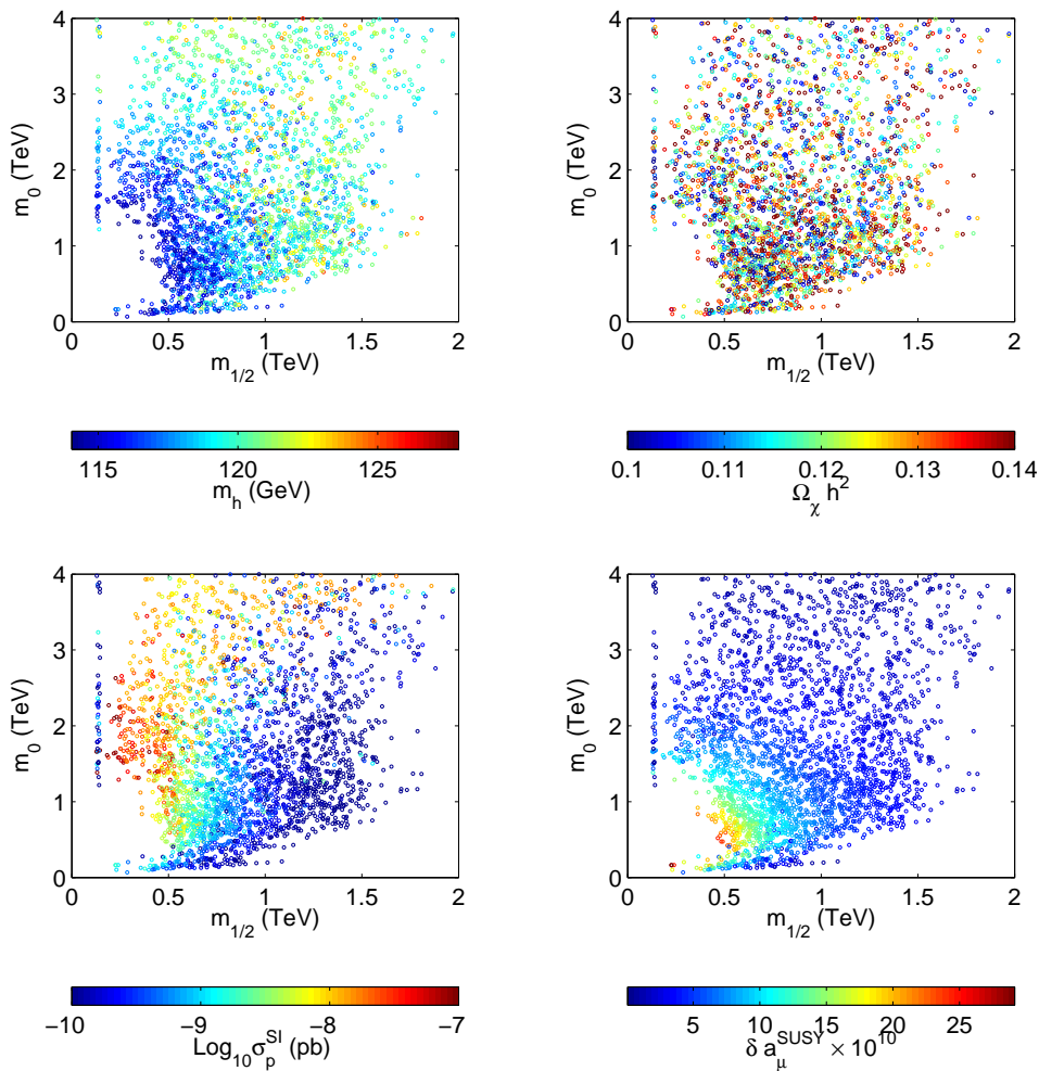
Figure 15: Values of m_h (upper left), \Omega_\chi h^2 (upper right), \sigma_p^{SI} (lower left) and \delta a_\mu^{\text{SUSY}} (lower right) in the (m_{1/2}, m_0) plane for samples uniformly selected from our MC chains. While \sigma_p^{SI} and \delta a_\mu^{\text{SUSY}} show a clear correlation with the values of (m_{1/2}, m_0) , the CDM abundance \Omega_\chi h^2 can take any value within the 2\sigma WMAP range in the plane. Narrow “WMAP strips” in the (m_{1/2}, m_0) plane for fixed values of \tan\beta and A_0 thus disappear when these parameters are allowed to vary and all other parameters are correctly marginalized over.
